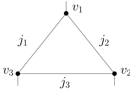
Figure 5: The tensor network graph of the tensor chain for d = 3 .
