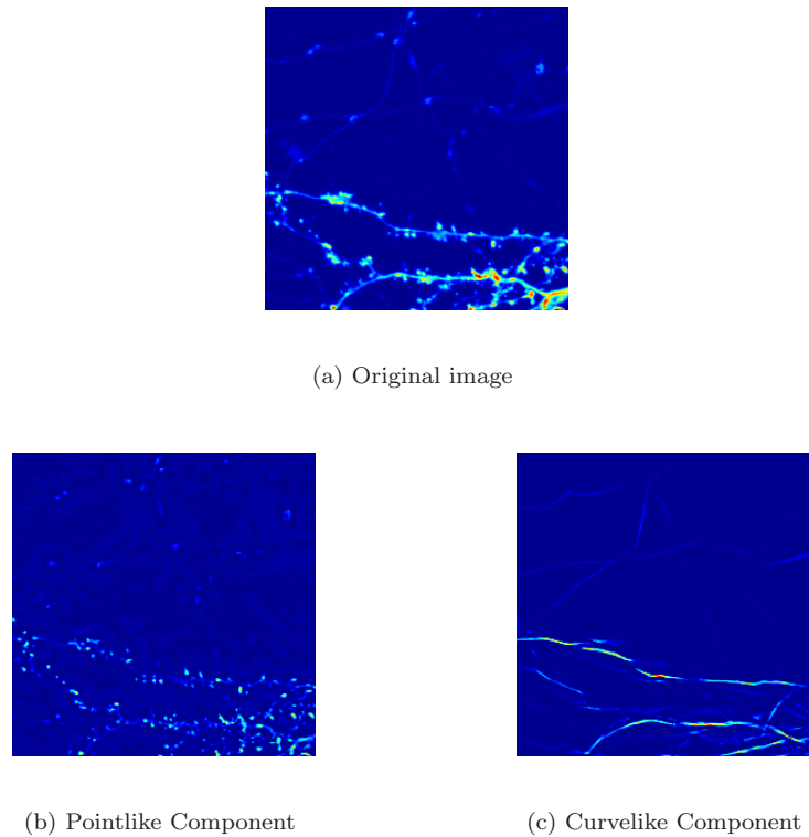
Figure 1.3 Separation of a neuron image into point- and curvelike components using ShearLab.
