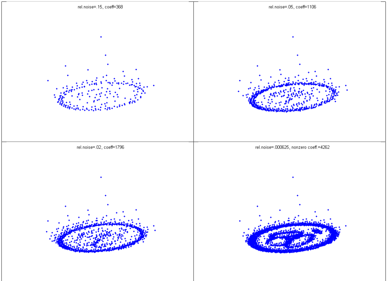
Figure 3: Different resulting wavelet frame grids associated to different adaptive reconstructions for noise levels \delta_{rel} = 15\% , 5\% , 2\% , 0.00625\% shown in Figure 2. The individual sub-figures are three-dimensional: the layer ordering is from coarse to fine scale frame coefficients (from top to bottom). Within each layer we have visualized the label/location of the frame coefficients (not its magnitude).
